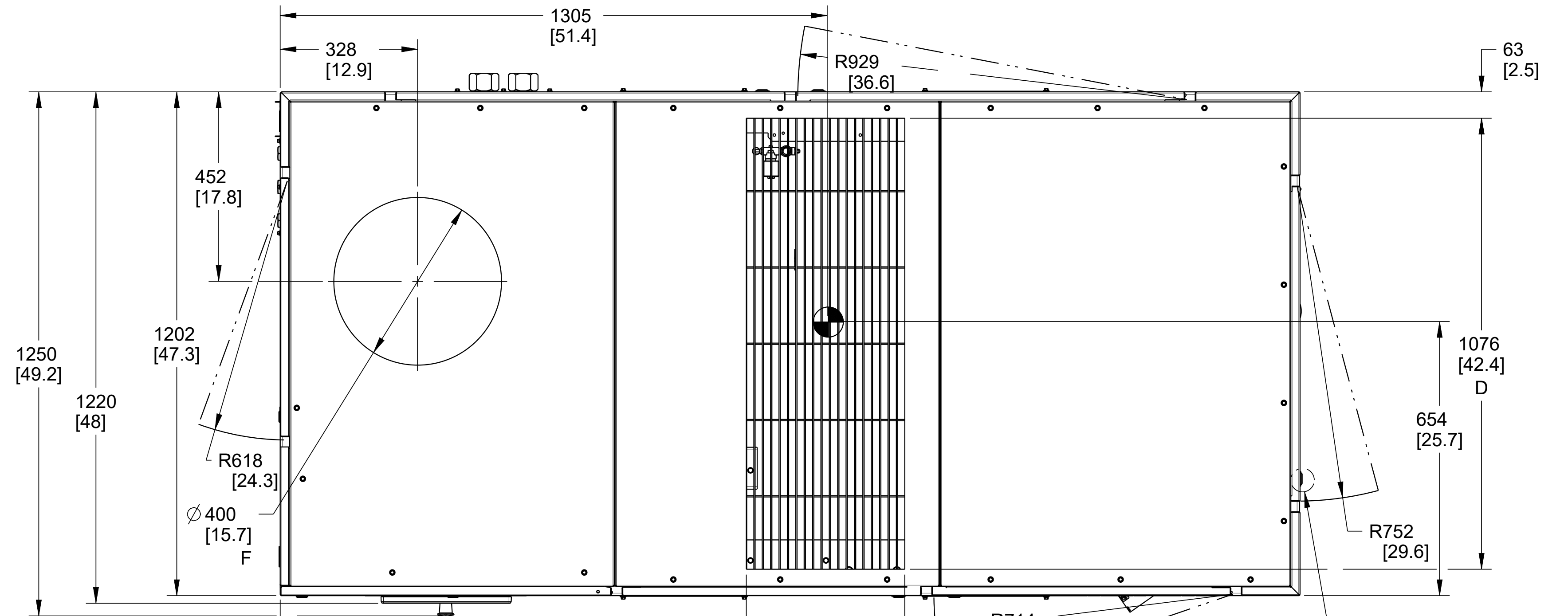
TOP VIEW
