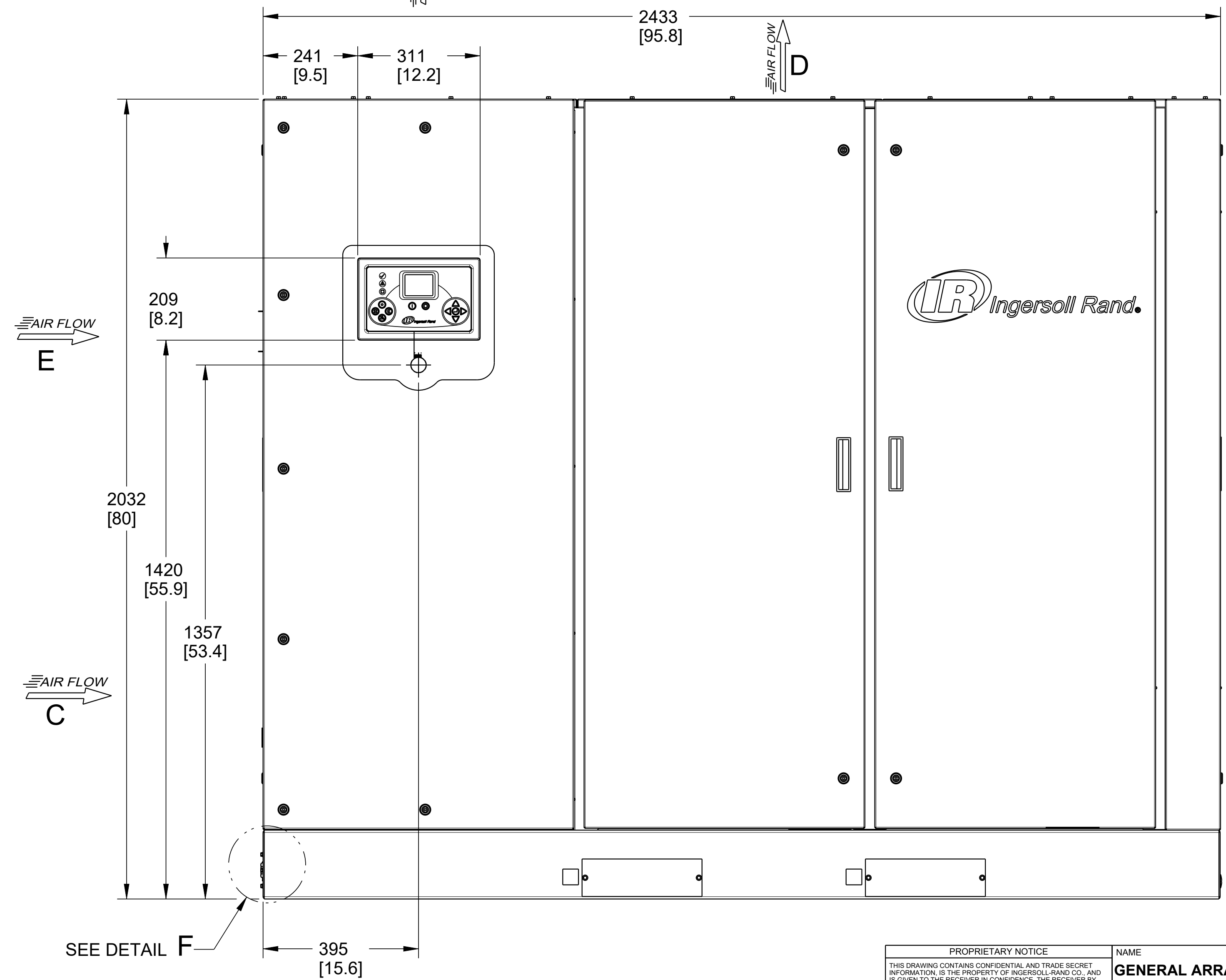
FRONT VIEW
