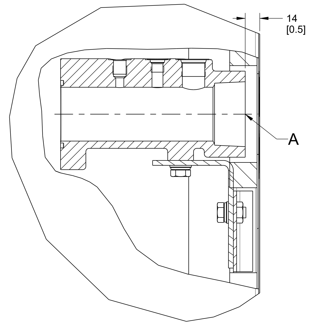
DETAIL D SCALE 0.600
