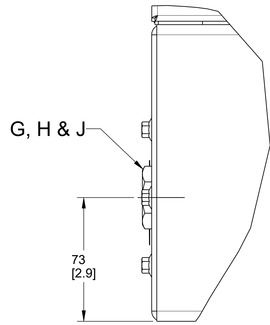
DETAIL F SCALE 0.750
