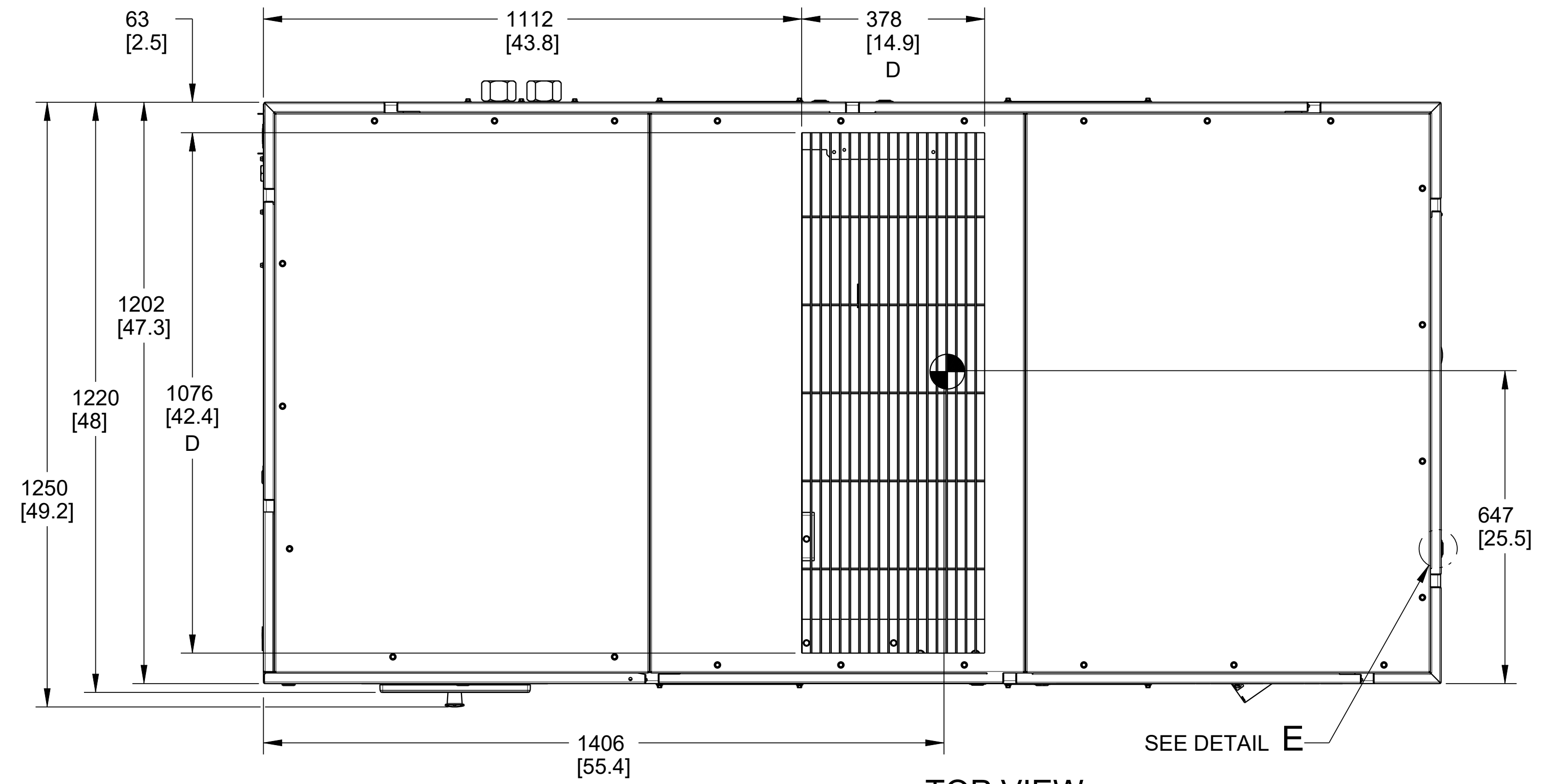
TOP VIEW
