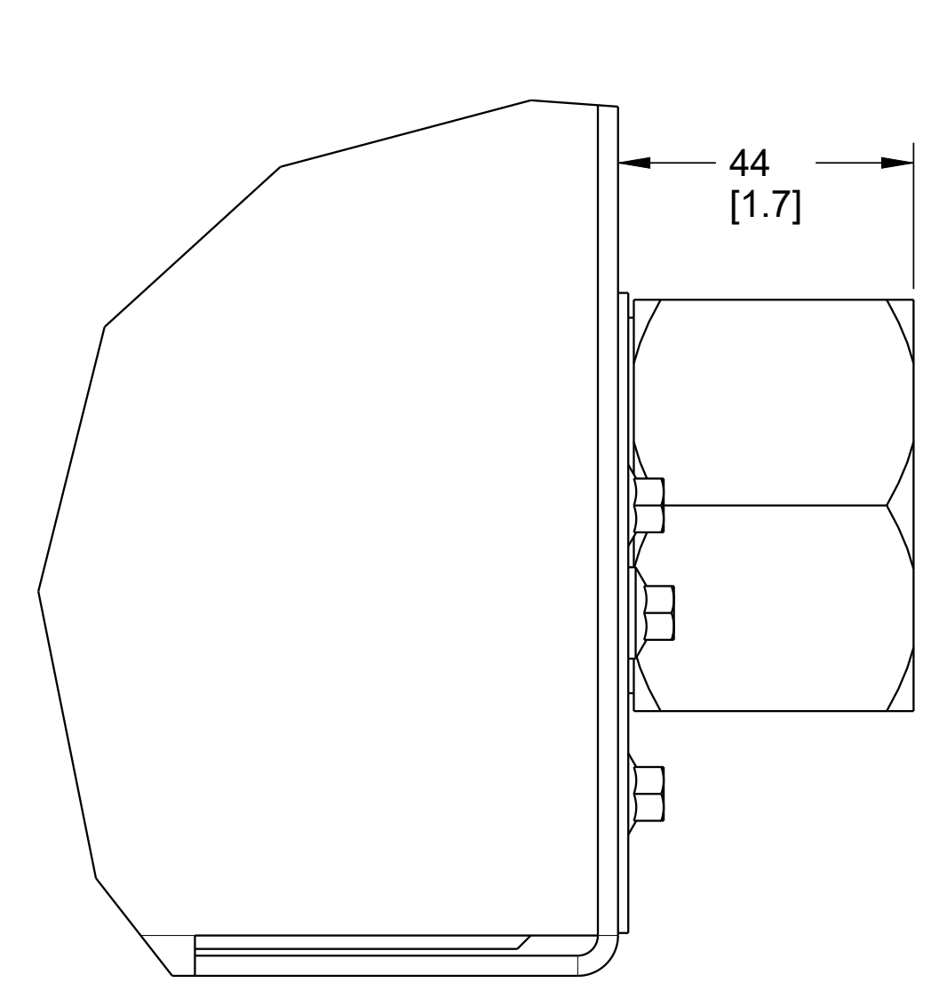
DETAIL C SCALE 1.000 (ERS OPTION ONLY)
