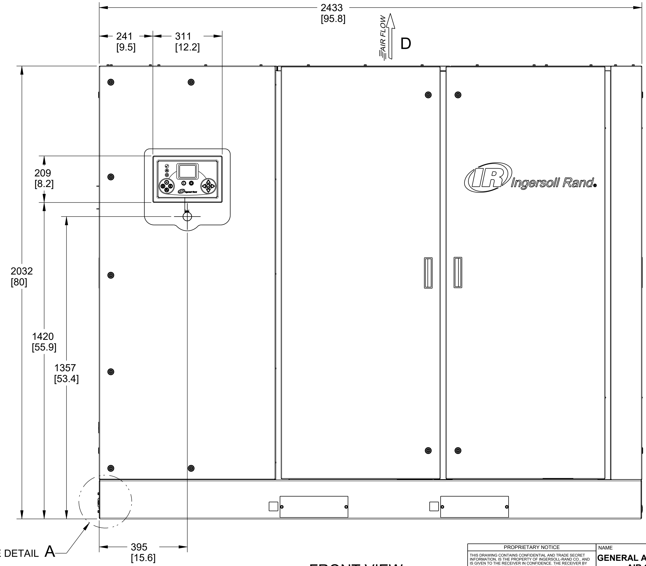
FRONT VIEW
