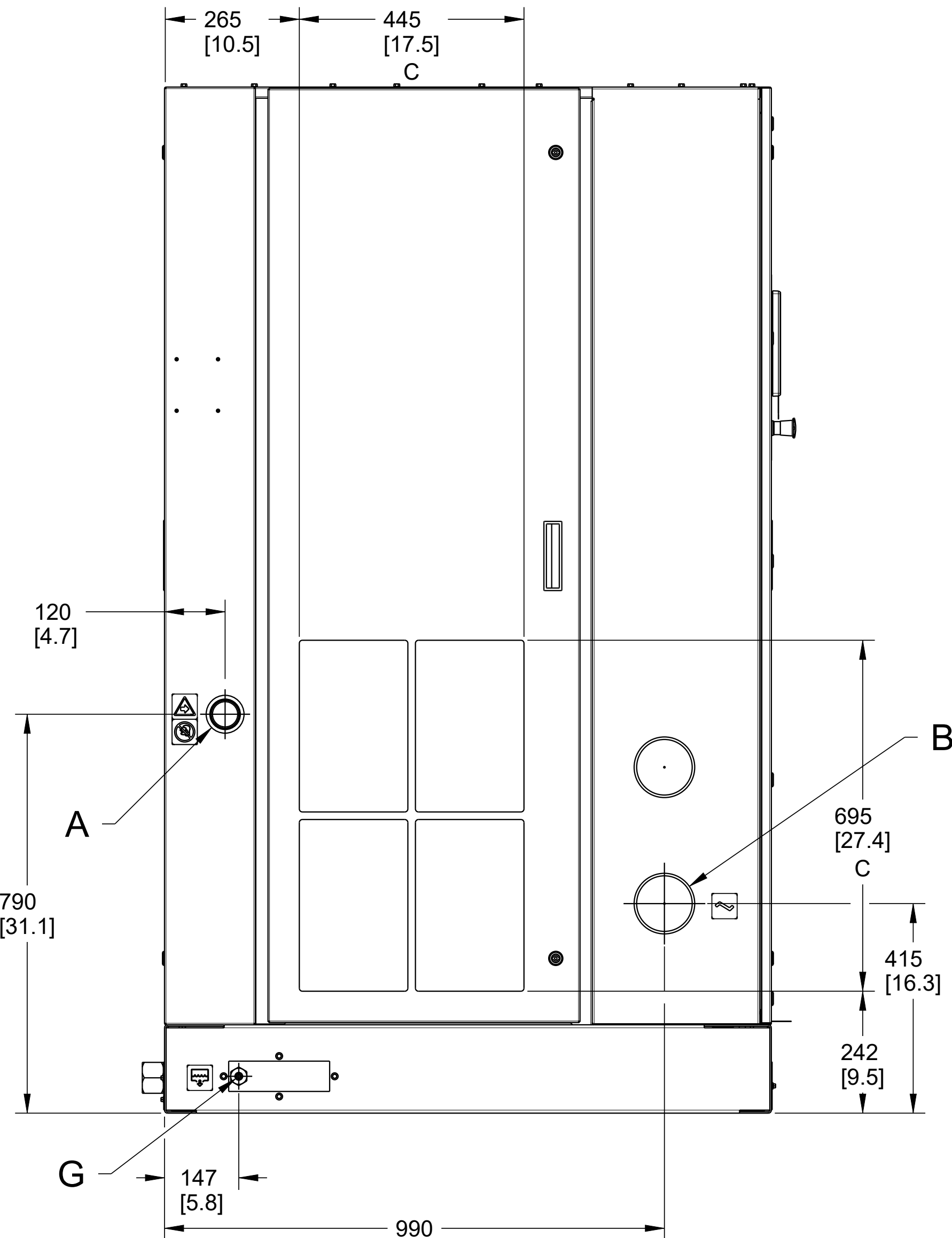
LEFT END VIEW
