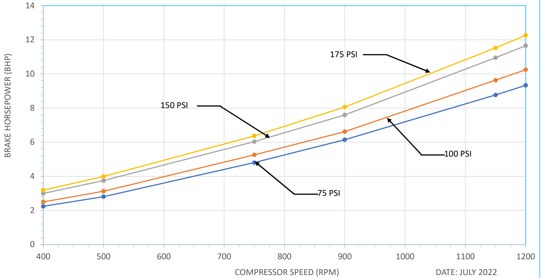
QT-1/QP-1 TYPICAL PERFORMANCE COMPRESSOR SPEED VS. BRAKE HORSEPOWER RPM RANGE 400 - 1200 MAX. PRESSURE 175 CONTINUOUS
