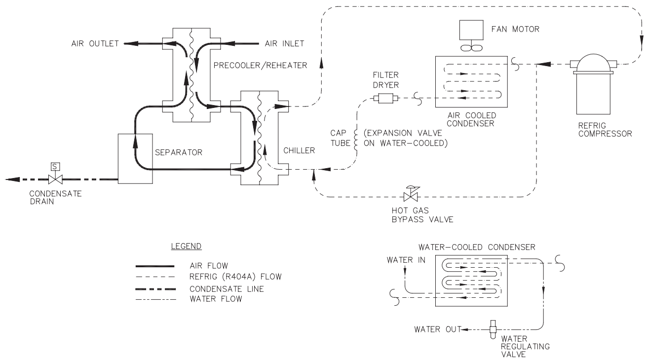
Figure 1 - Flow Diagram
