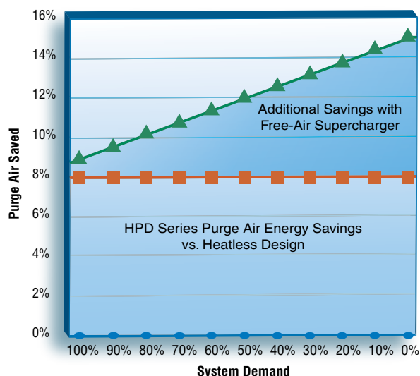
▲ HPD Series and EMS with Free-Air Supercharger (6% purge) ■ HPD Series (standard 7% purge) ● Heatless Design (Industry average 19% purge)
