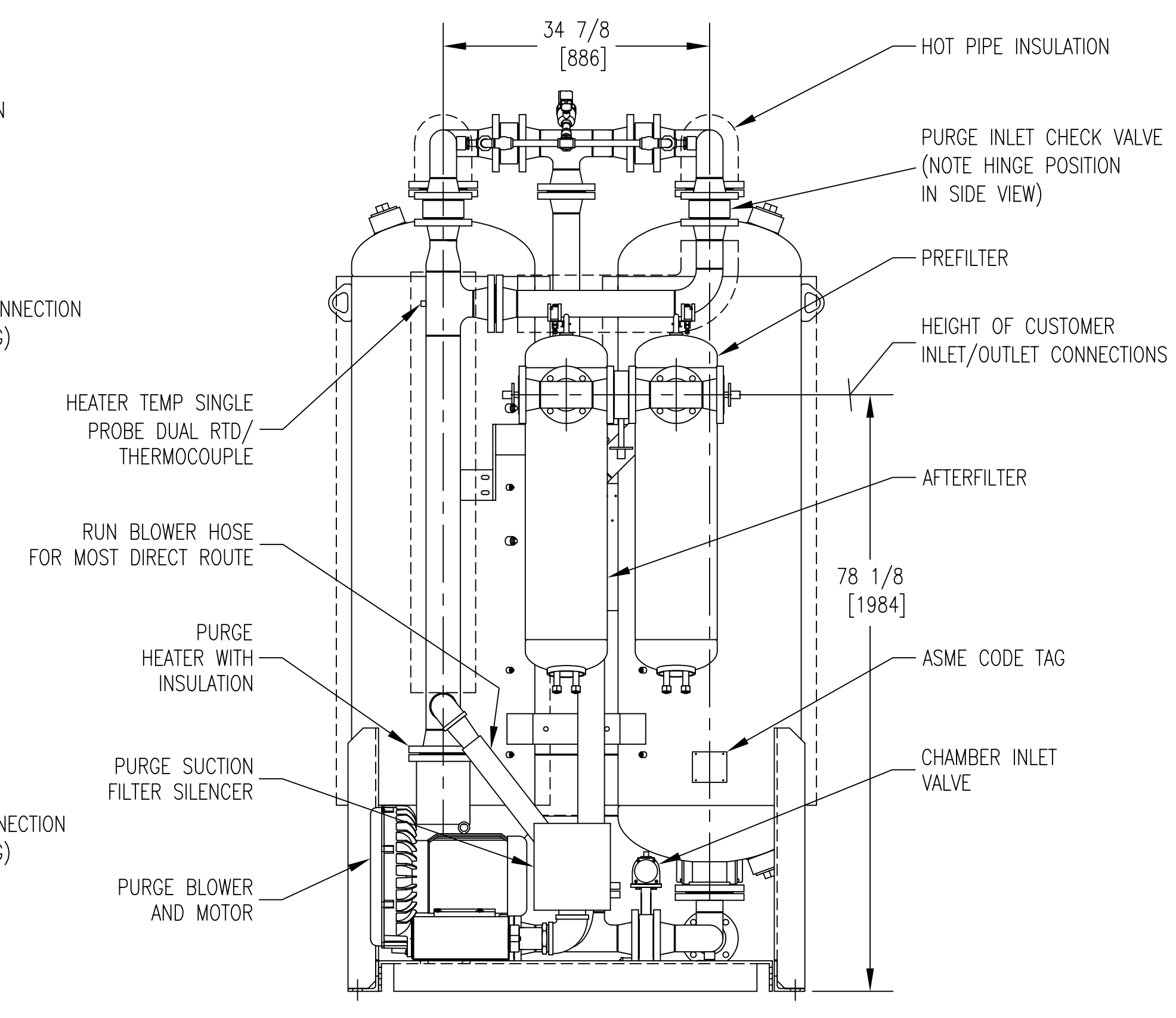
REAR VIEW (F01/F02 PKG OPTIONAL)
